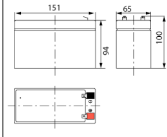
Dimensions (mm)
