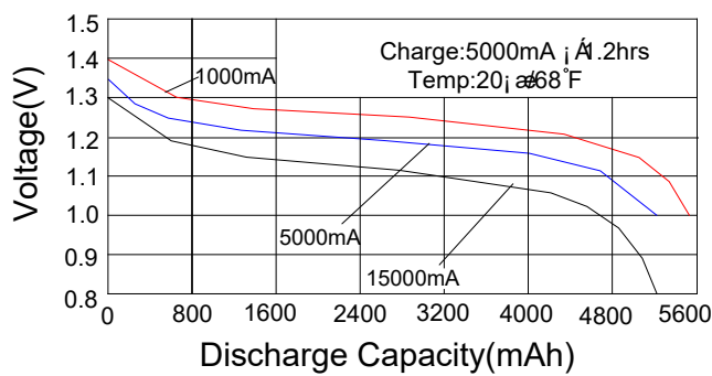
Discharge characteristics
